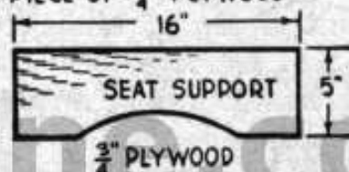
SEAT AND CENTER SECTION ARE CUT FROM ONE PIECE OF 3/4" PLYWOOD
