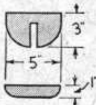
CENTER SECTION LOCK PIECES 3/8" PLYWOOD (2 - 3"x5" AND 4 - 1"x5" PIECES NEEDED)
