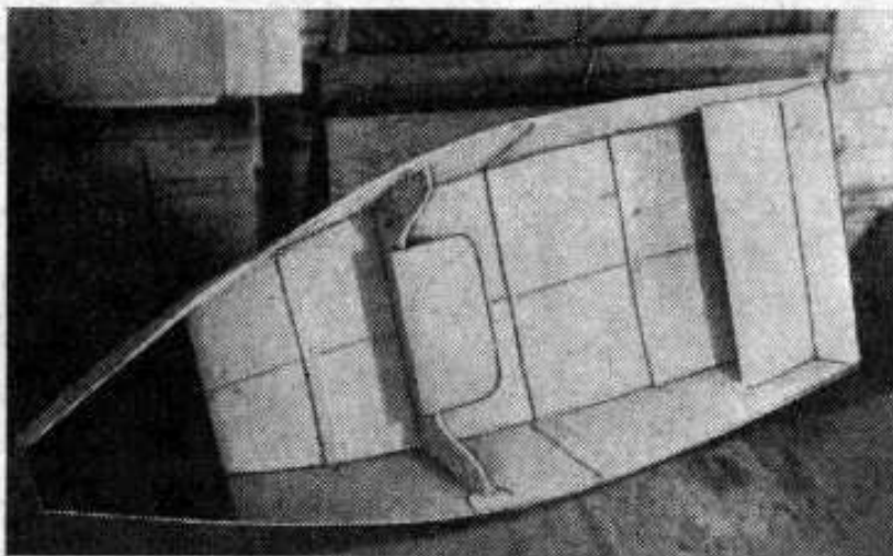
The completed boat with a canvas "deck" stretched across the bow. Removable center section with seat, the plywood transom, and the transom seat hold the boat rigid when it is opened up. The parts named can be taken out or installed quickly.
